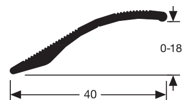
ALUMINIUM PERCÉE
