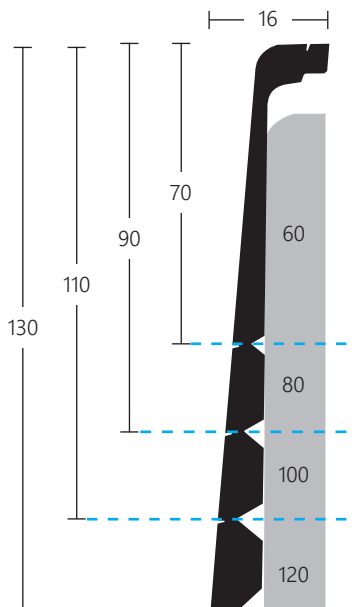
Surplinte universelle
